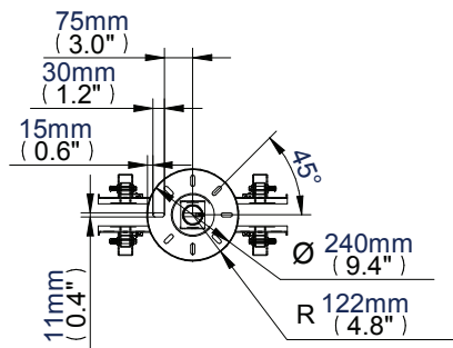
Ceiling Plate
