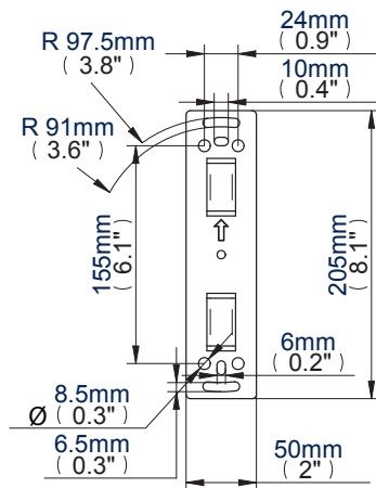
Wall Plate
