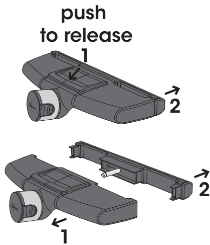
1 Flex Mount
