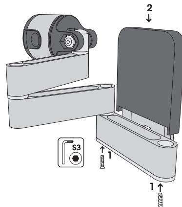
4 Flex Mount
