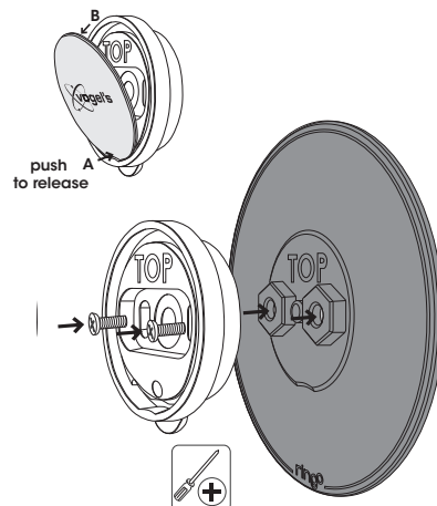
B4 Thin Mount / Adhesive
