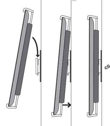
Thin Mount Usage
