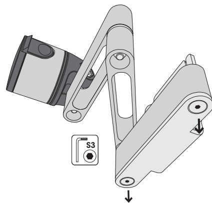
B2 Thin Mount / Adhesive
