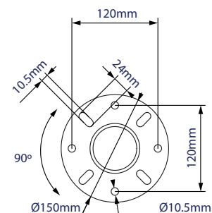
Ceiling Plate
