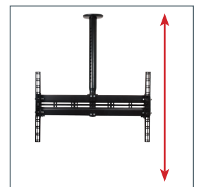
Ceiling drop: 668mm - 993mm in 25mm (1") increments
