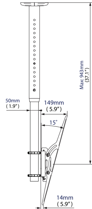
Side View - Maximum Drop
