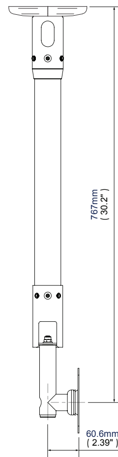
BT7553-050 Side View
