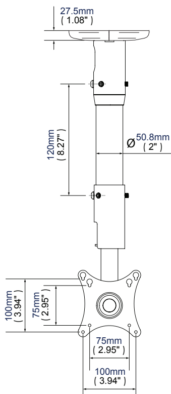
BT7553-025 Front View
